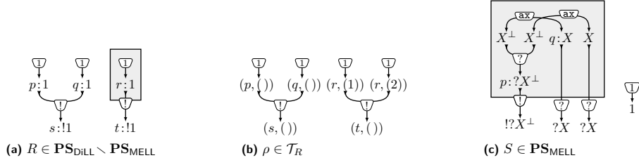
■ Figure 8 A box-connected DiLL-ps R (Fig. 8a, with \mathcal{C}_R^{\text{box}} = \{l\} and \mathcal{C}_R \setminus \mathcal{C}_R^{\text{box}} = \{o\} ) and a 2-diffnet \rho (Fig. 8b) of R (see also Remark 26). Moreover, a box-connected MELL-ps S (Fig. 8c).
