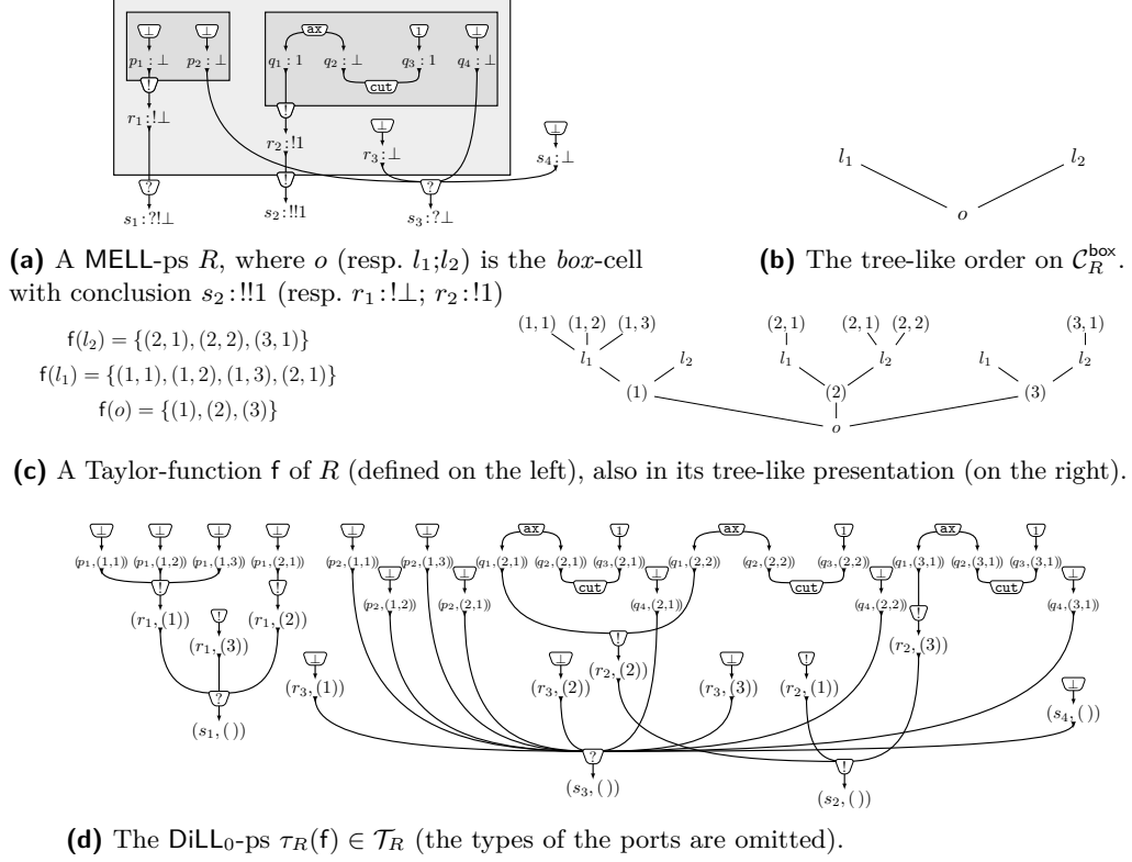
■ Figure 4 From a MELL-ps R (Fig. 4a) to an element of the labeled Taylor expansion of R (Fig. 4d), via a Taylor-function of R (Fig. 4c). See also Example 15.
