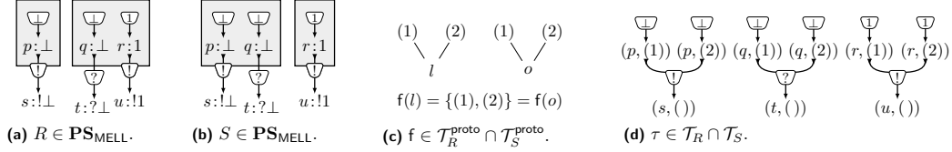
■ Figure 6 Two non-isomorphic MELL-ps R (Fig. 6a) and S (Fig. 6b), where l (resp. o ) is the box -cell of R and S with conclusion s:!!1 (resp. u:!!1 ). The DiLL 0 -ps \tau \in \mathcal{T}_R \cap \mathcal{T}_S (Fig. 6d) is the 2-diffnet of R and S generated by the Taylor-function f of R and S (Fig. 6c), i.e. \tau_R(f) = \tau = \tau_S(f) .
